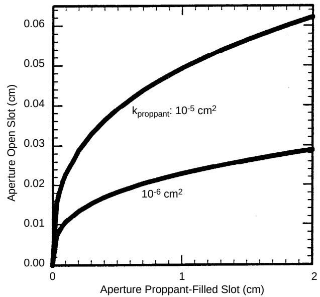
Figure 3-12. Effective aperture of an open slot that is equivalent to that of a fracture filled with proppant.
