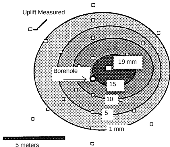
Figure 3-3. Typical pattern of uplift over a shallow, gently dipping hydraulic or pneumatic fracture.
