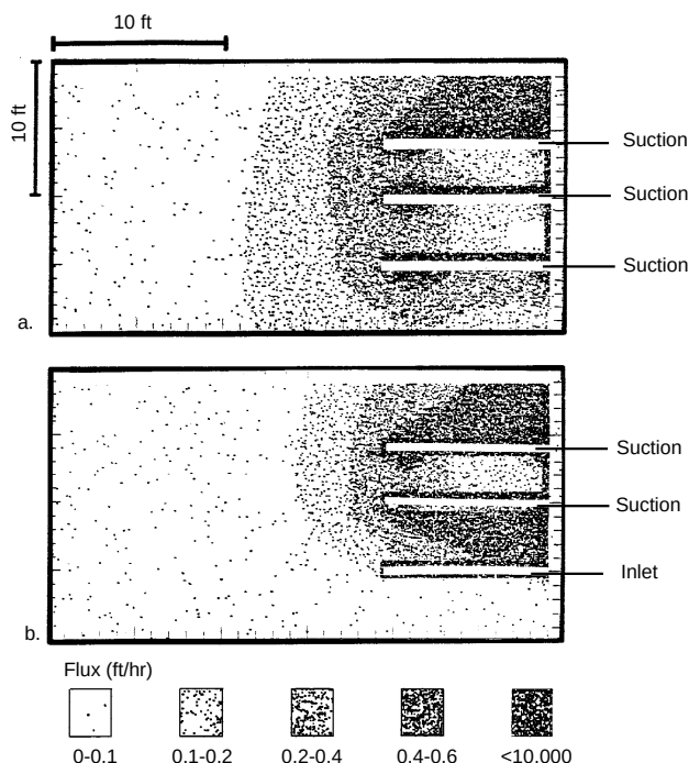
Figure 3-14. Flux of air to three flat-lying fractures (white band) shown in cross section: a) suction of 100 inches of water on all three fractures, and b) air inlet (atmospheric pressure) at the bottom and suction on the other two fractures.
