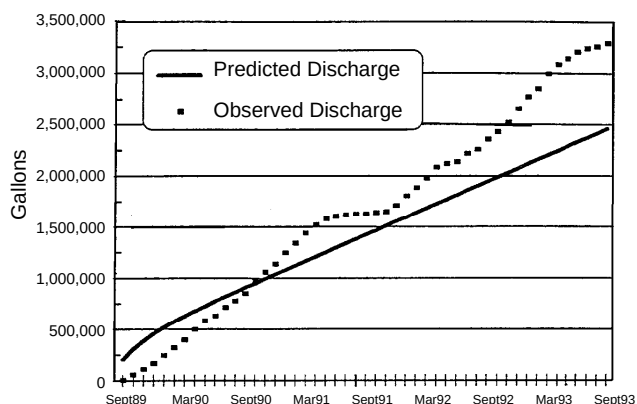
Figure 4-27. Observed and predicted discharges from trench system.
