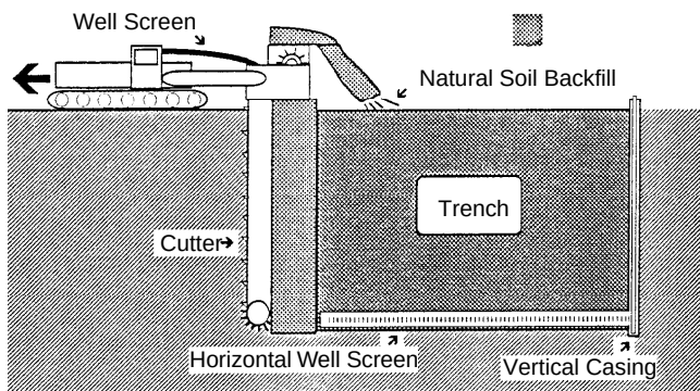
Figure 4-2. Schematic of continuous excavation and completion technique (6).
