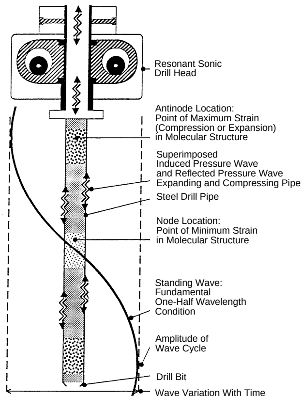
Figure 2-6. Resonant stress wave providing energy to the drill bit (10).
