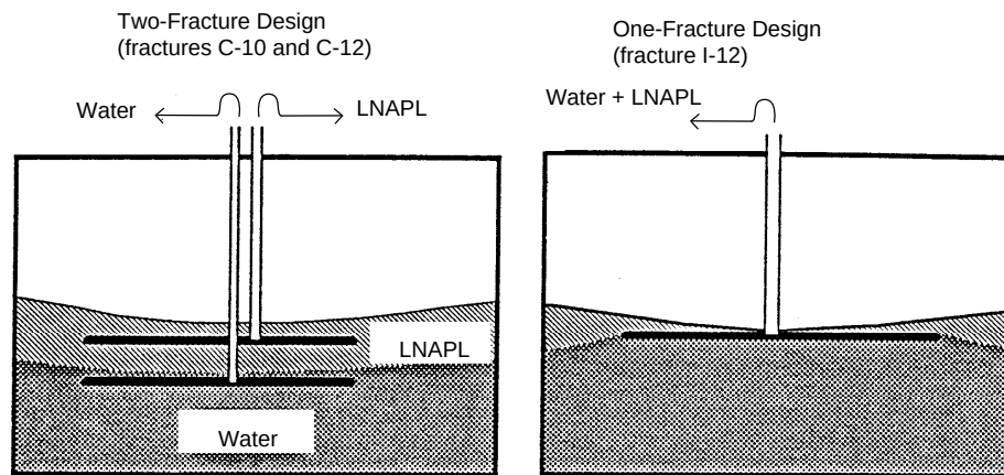
Figure 3-19. Methods of completing a well containing hydraulic fractures to recover LNAPL.
