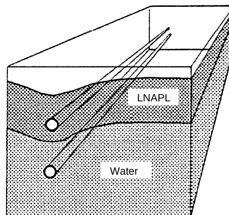
Figure 2-20. Recovery of LNAPL with one horizontal well, and water control with another well below.
