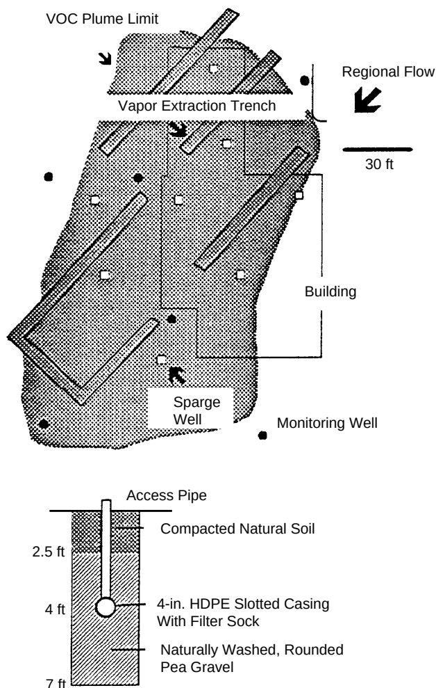
Figure 4-18. Map of the northeastern Illinois vapor extraction site and detail of trench completion (24).
