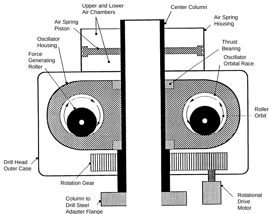
Figure 2-7. Sonic drill head (10).
