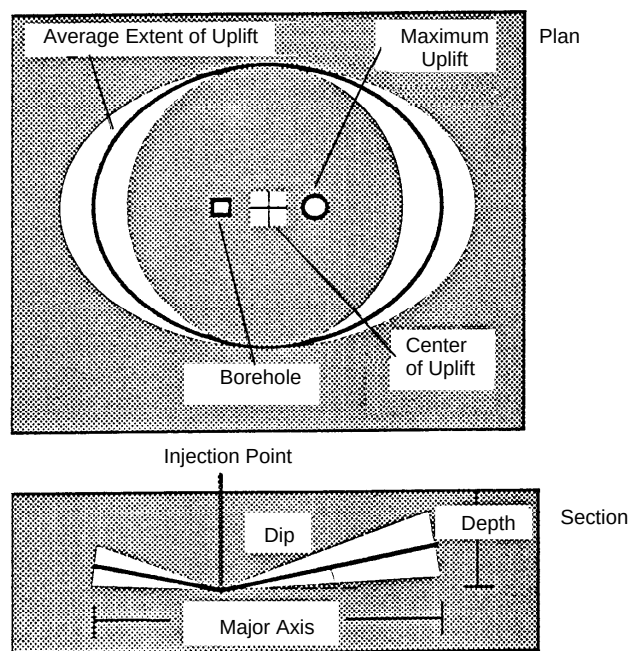
Figure 3-10. Plan and section of a typical hydraulic fracture created in overconsolidated silty clay.
