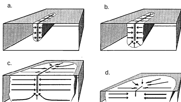
Figure 4-4. The pattern of flow to a trench with no regional gradient: a) linear flow, b and c) transition, and d) radial flow (11).
