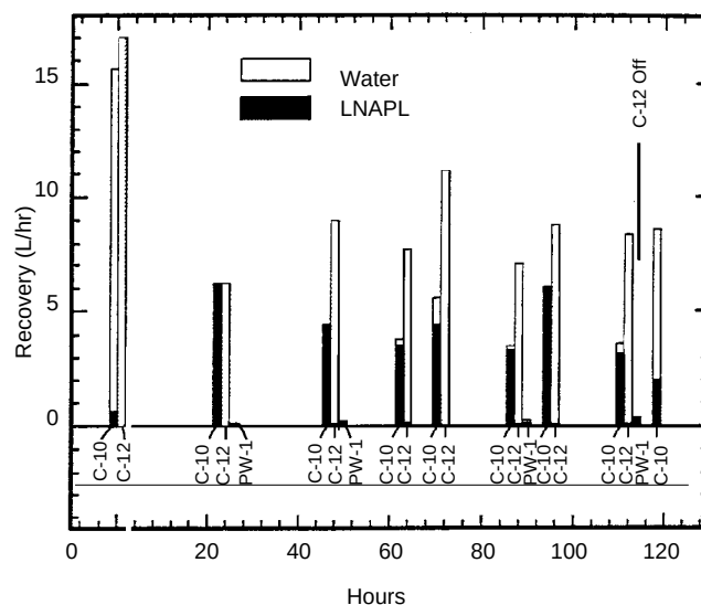
Figure 3-20. Discharges from C-10, C-12, and PW-1 as functions of time.
