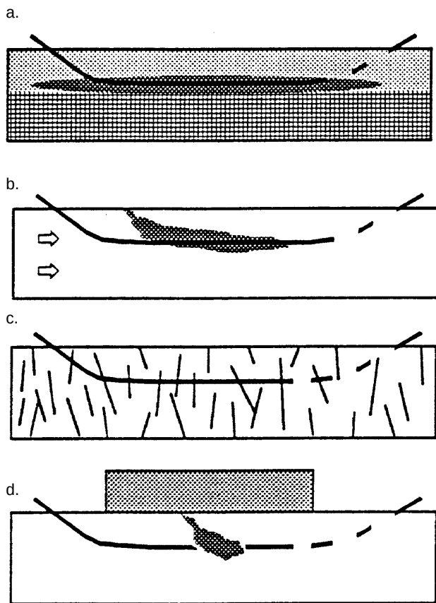
Figure 2-2. Some applications of horizontal wells: a) intersecting flat-lying layers, b) intercepting plume elongated by regional gradient, c) intersecting vertical fractures, and d) access beneath structures.
