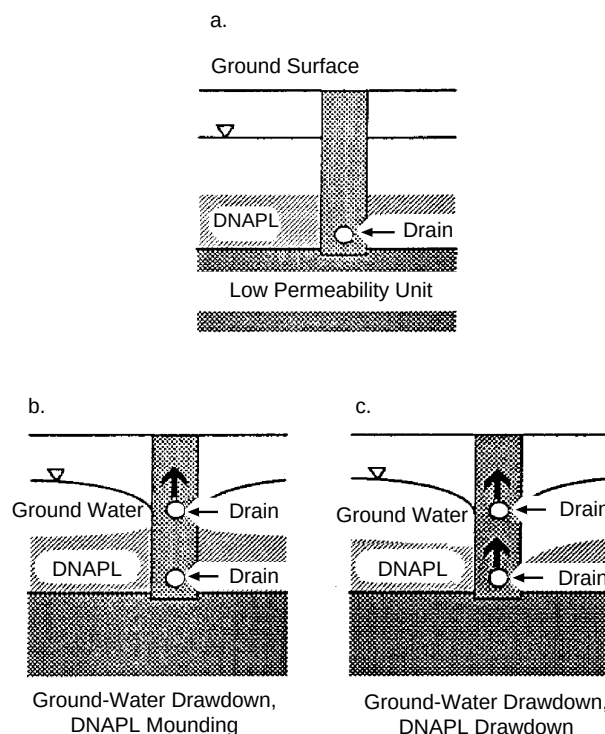
Figure 4-13. Trench systems for DNAPL recovery: a) one-drain system, b) two-drain system with upper drain pumping, and c) two-drain system with both drains pumping (22).
