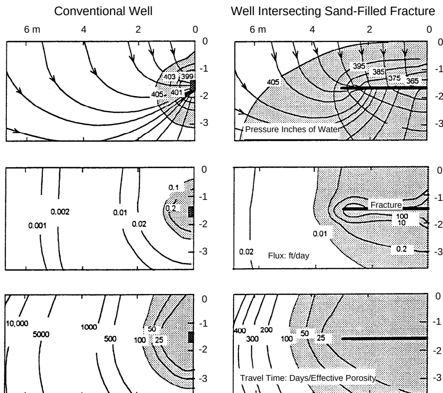
Figure 3-9. Pressure, flux, and travel time to a conventional well and a well intersecting a sand-filled fracture. Shaded areas are for comparison (based on the results of a numerical simulation using field data [22]).
