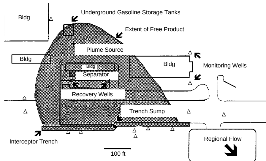
Figure 4-16. Plan of the Westminster gasoline recovery site (15).
