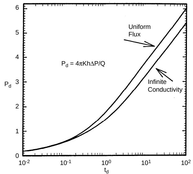
Figure 4-5. Drawdown at the midpoint of a trench where discharge is constant (11).
