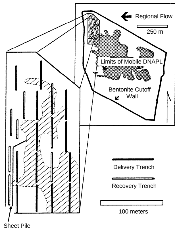
Figure 4-17. Plan of the Laramie DNAPL recovery site (20).
