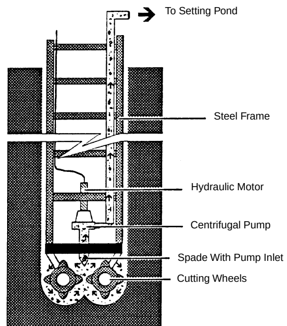
Figure 4-3. Schematic of deep trench excavation equipment (redrawn from material provided by Coastal Caisson Corp., Clearwater, FL).
