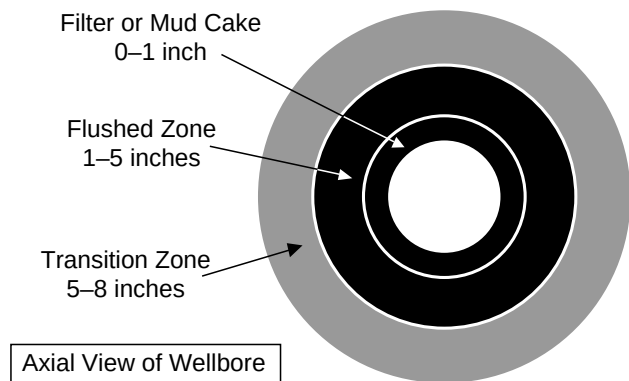
Figure 2-5. Potential damaged zones around a horizontal wellbore.
