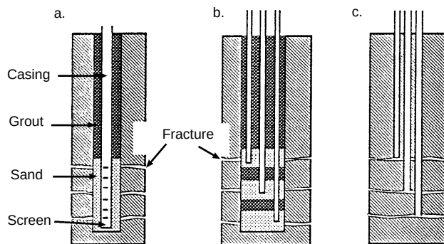
Figure 3-7. Methods of completing wells with induced fractures: a) screen across all fractures b) casing to each fracture, and c) driven casing to each fracture.
