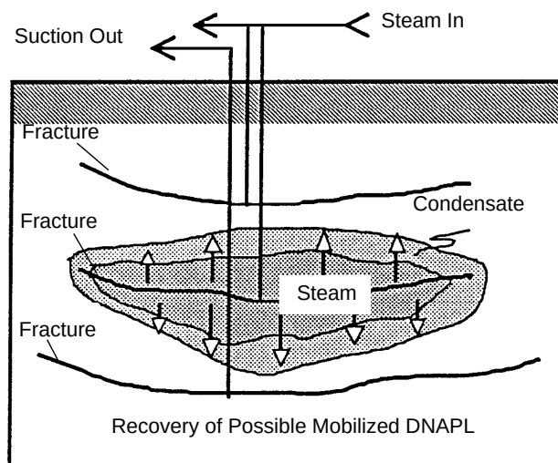
Figure 3-16. Schematic application of steam injection into induced fractures.
