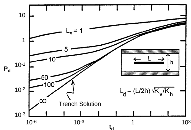
Figure 2-15. Drawdown resulting from a horizontal well as a function of time and dimensionless length. Drawdown and time are dimensionless.
