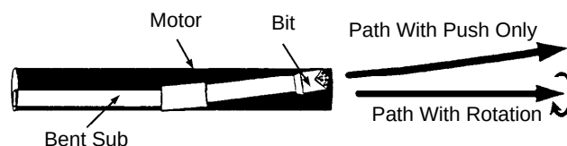
Figure 2-4. Directional drilling with a downhole motor.
