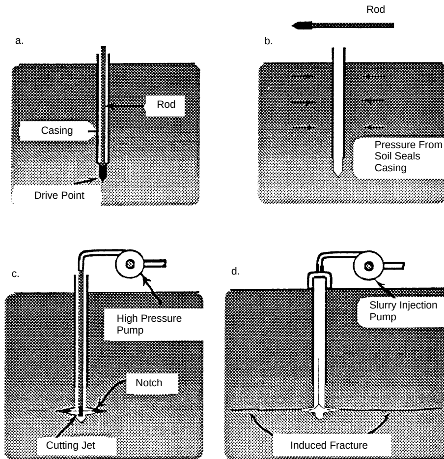
Figure 3-6. Fractures created at the bottom of driven casing.
