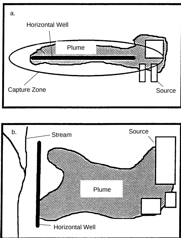
Figure 2-18. Two approaches using horizontal wells to intercept contaminant plumes.
