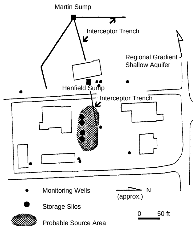
Figure 4-24. Site plan showing locations of initial interceptor trench segments (38).
