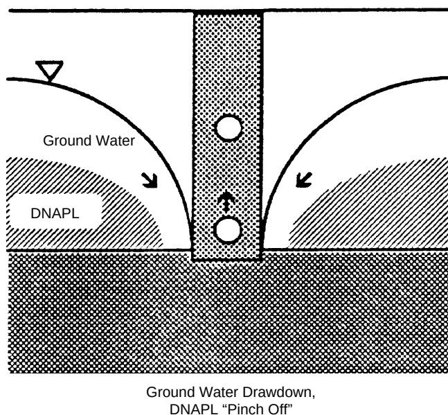
Figure 4-15. Excessive pumping rates from the ground-water and DNAPL drains causing “pinch off” of the DNAPL plume.
