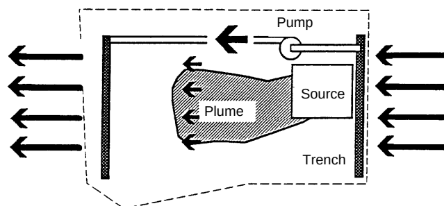
Figure 4-10. Controlling the flow through a contaminated area by pumping from an upgradient trench and injecting into a downgradient trench.
