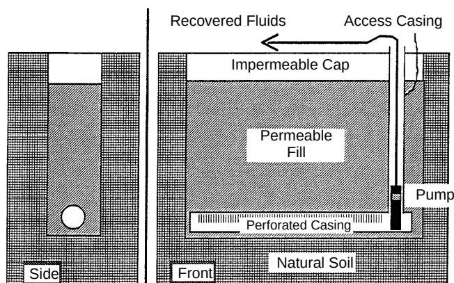
Figure 4-1. Cross sections of a basic interceptor trench configuration showing permeable backfill and perforated casing.
