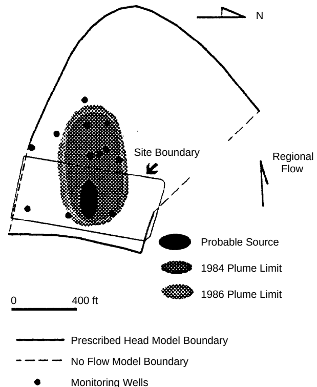
Figure 4-21. Extent of TCE plume in 1984 and 1986; also shown is the ground-water model domain, with prescribed (fixed) head and no-flow boundaries (34).
