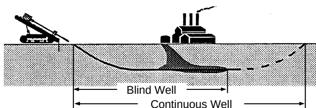
Figure 2-1. Horizontal well used to intercept a plume. The solid line represents a blind well; the solid line plus the dashed line represents a continuous well.
