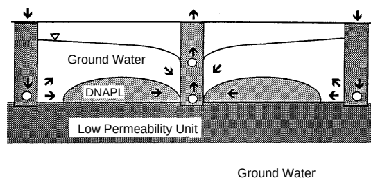
Figure 4-14. Enhanced recovery of DNAPL by reintroducing water to increase the hydraulic gradient (20).
