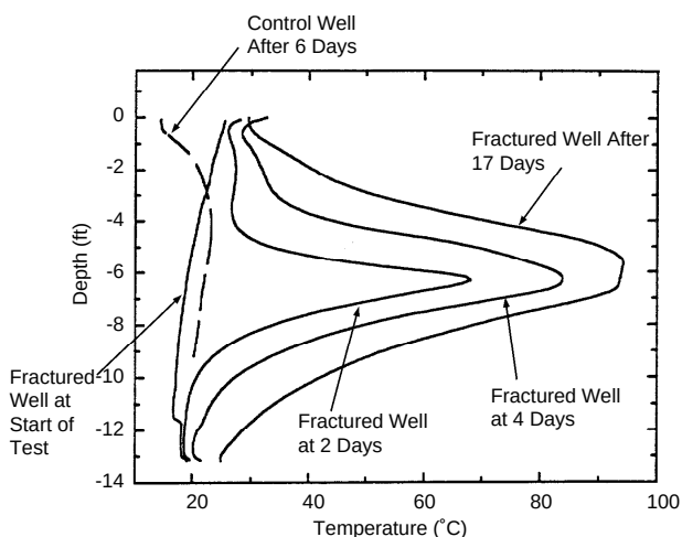
Figure 3-17. Temperature as a function of depth and time.
