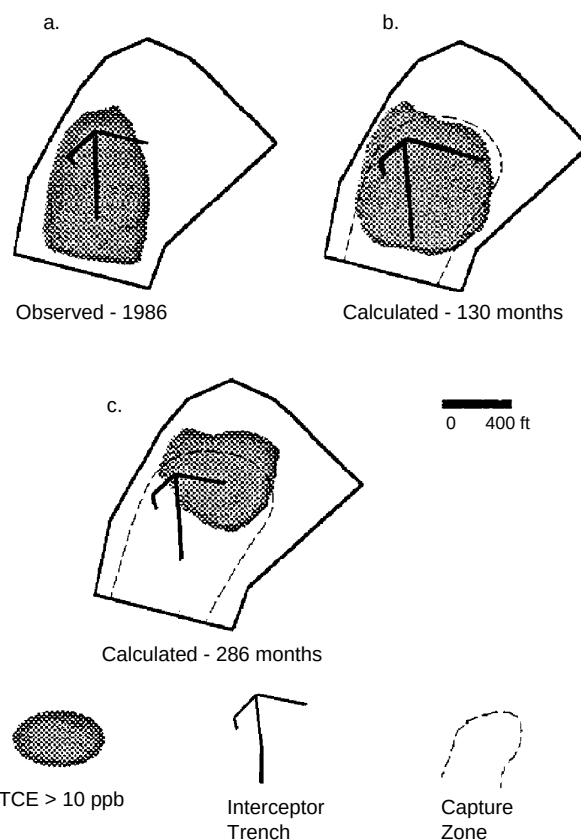
Figure 4-23. TCE concentration distribution through time (Note: TCE >10 ppb outside of capture zone.)
