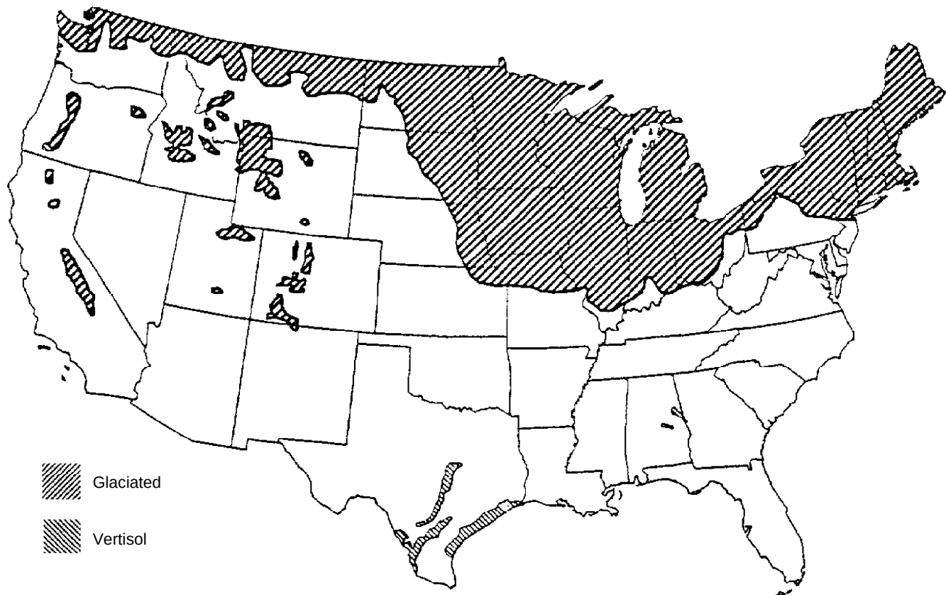
Figure 3-11. Locations of major areas of soils related to glaciers and vertisols (25, 26).
