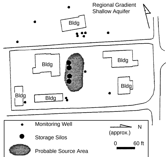
Figure 4-20. Site map showing locations of monitoring wells, storage silos, and probable contaminant source area (34).
