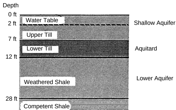
Figure 4-19. Typical subsurface profile (34).
