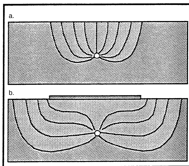
Figure 2-19. Schematic of flow patterns with horizontal wells: a) without cap and b) with cap.
