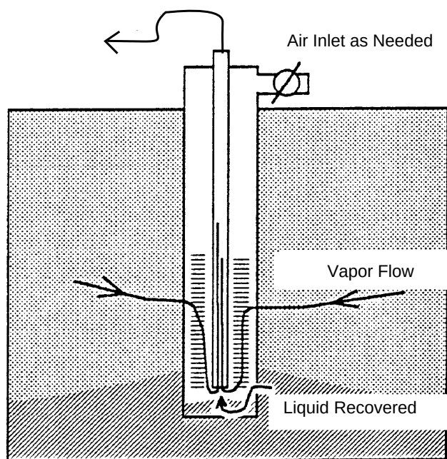
Figure 3-15. Well configuration to recover liquid and vapor phases using suction at the ground surface.
