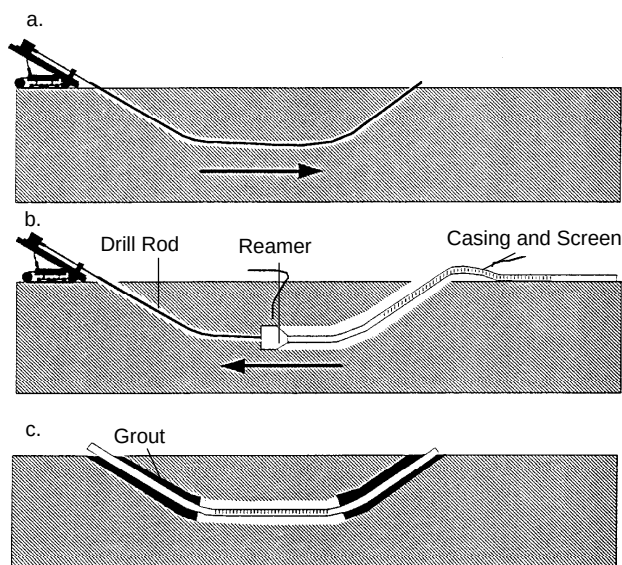
Figure 2-8. Creating a horizontal well with the pull-back method: a) drilling a continuous wellbore, b) reaming and pulling in casing, c) the finished well.
