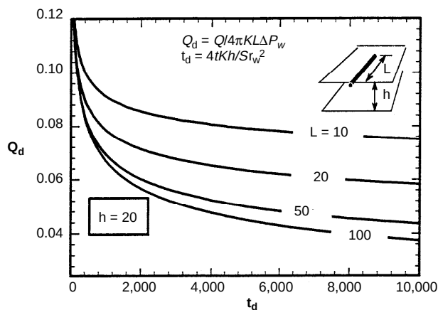
Figure 2-16. Discharge from horizontal wells of different lengths operated at constant drawdown (24).
