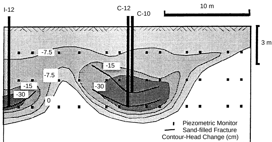
Figure 3-21. Cross section along line of piezometers showing change in head after 5 days of pumping.
