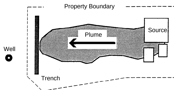
Figure 4-12. Trench used to capture plume and prevent migration to an offsite well.
