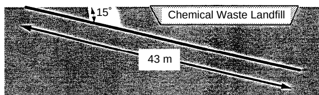
Figure 2-21. Inclined wellbore created with resonant sonic drilling, Sandia National Laboratories (38).
