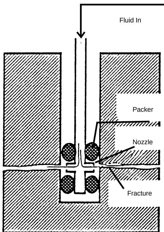
Figure 3-5. Fracture created by isolating a zone with a straddle packer.
