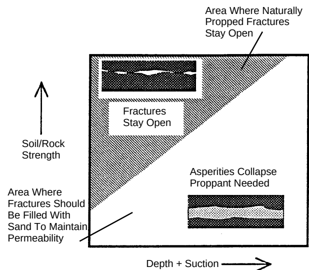
Figure 3-13. Factors that affect how fractures should be propped.
