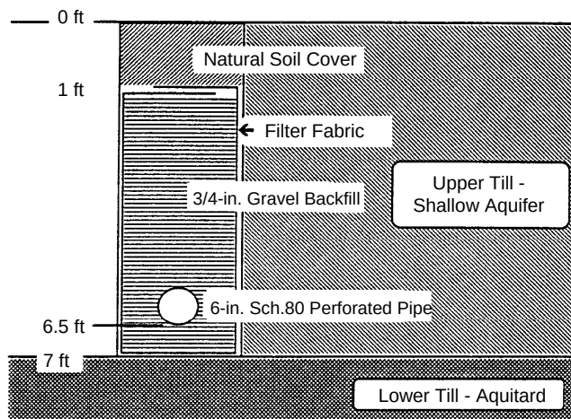
Figure 4-25. Schematic cross section of trench construction (38).
