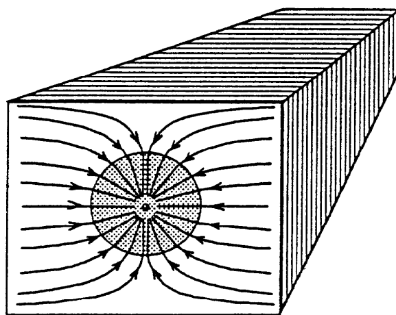
Figure 2-12. Radial flow in a vertical plane in the vicinity of a horizontal well.
