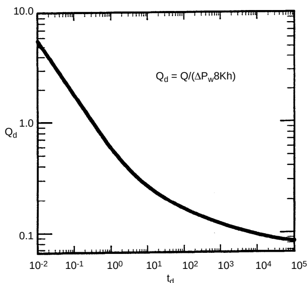
Figure 4-6. Discharge from a trench held at constant drawdown (11).
