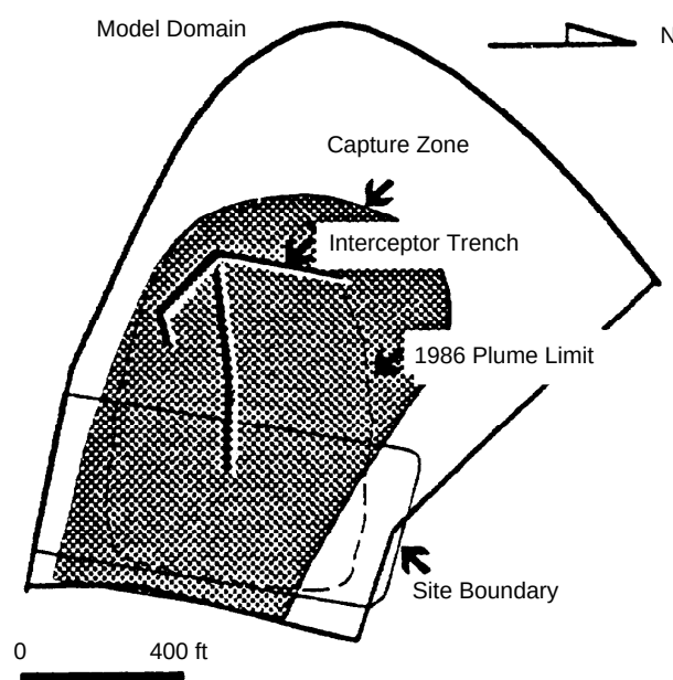
Figure 4-22. Model domain showing location of the interceptor trench, the 1986 TCE plume limit, and extent of the capture zone (34).
