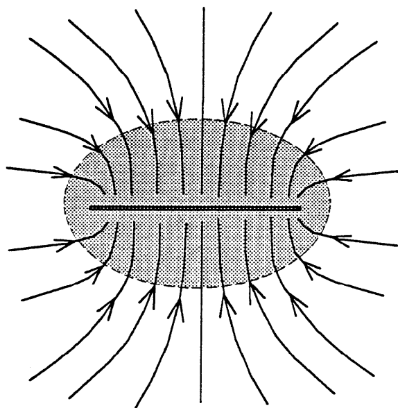
Figure 2-11. Flow paths to a horizontal well in a thin aquifer with no regional flow. Lines are nearly straight and parallel within the patterned area.
