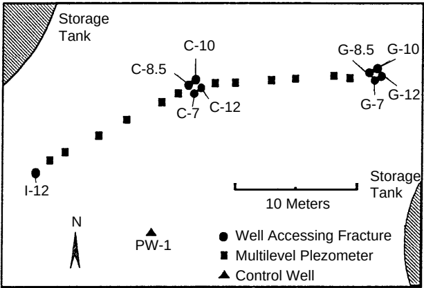
Figure 3-18. Area of LNAPL recovery using fractured and conventional wells.
