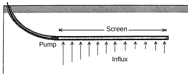
Figure 2-17. Schematic of distribution of influx into a horizontal well.
