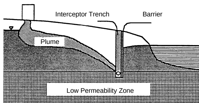
Figure 4-11. Interceptor trench coupled with a hydraulic barrier to minimize recharge from an adjacent surface waterbody.
