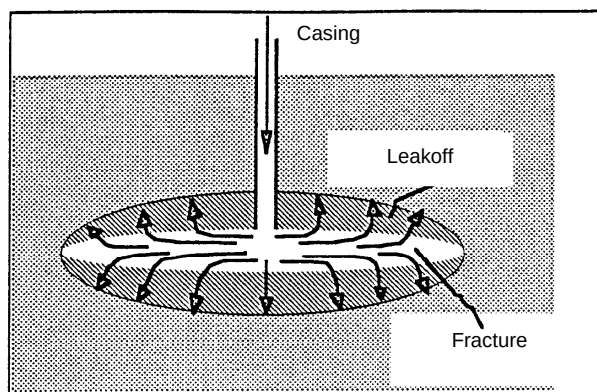
Figure 3-2. Injected fluids leaking out of fracture during propagation.
