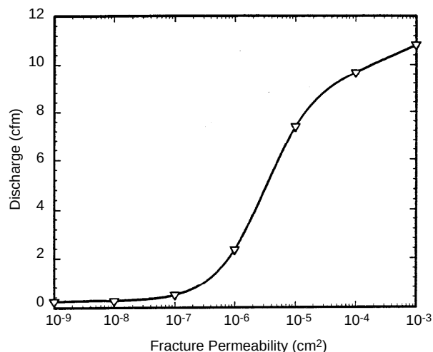
Figure 3-8. Air discharge from a well intersecting a flat-lying circular fracture as a function of the permeability of the fracture. (Formation permeability is 10^{-9} cm².)
