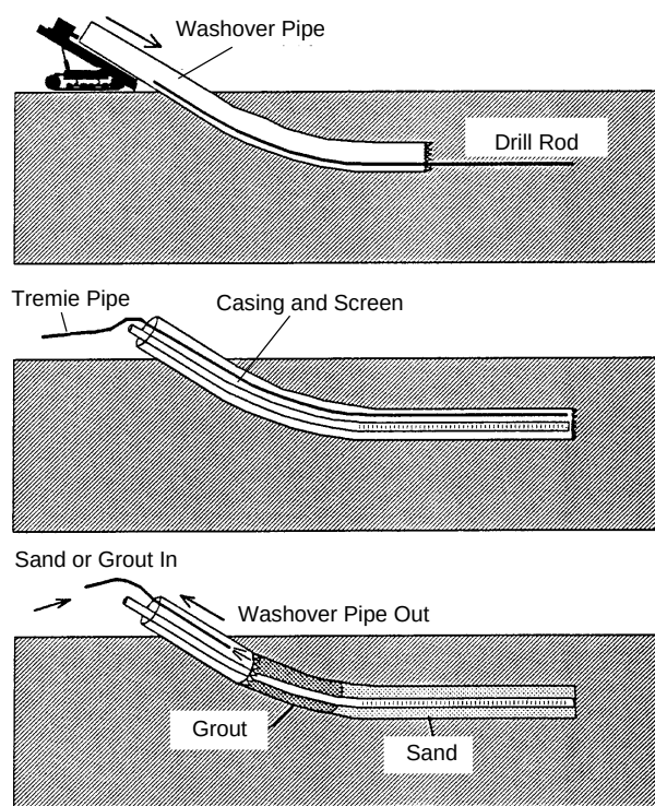
Figure 2-9. Completing a blind well using the washover pipe method.
