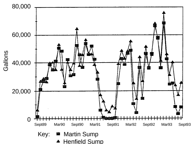
Figure 4-26. Monthly extraction from interceptor trench sumps.
