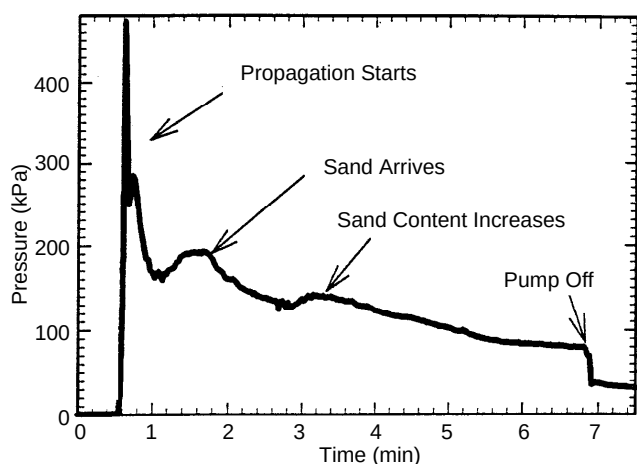
Figure 3-1. Injection pressure during creation of a fracture by injecting a sand-laden slurry.
