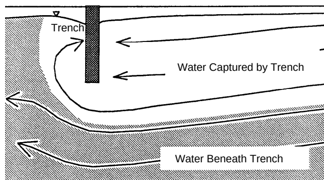
Figure 4-7. Cross section of a trench partially penetrating an aquifer in a regional flow, showing the vertical extent of aquifer captured by the trench.
