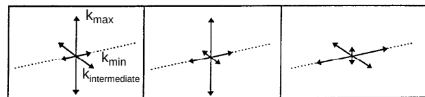
Figure 2-14. Orientations of horizontal well (dashed line) relative to principal directions of permeability.
