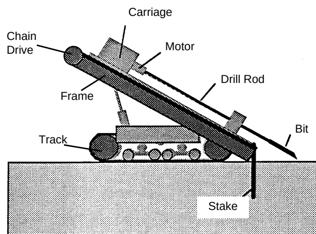
Figure 2-3. Directional drilling rig.
