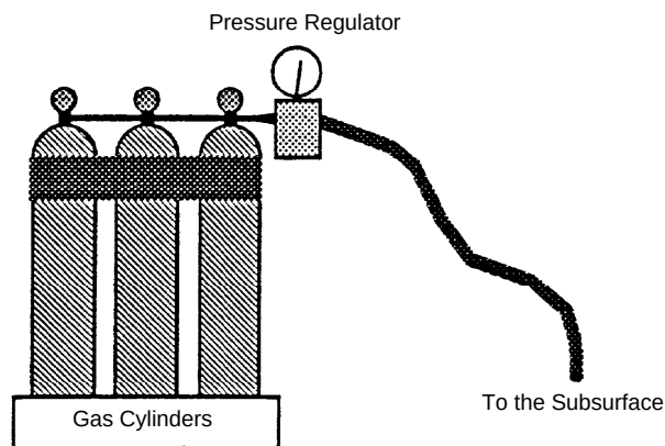
Figure 3-4. Aboveground equipment used for pneumatic fracturing (9).
